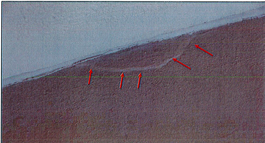
Photo #5. View of deteriorated ceiling stucco finishes, signs of concrete slab spalling due to corroded reinforcing, condition observed at floor of unit 504 front corridor.
