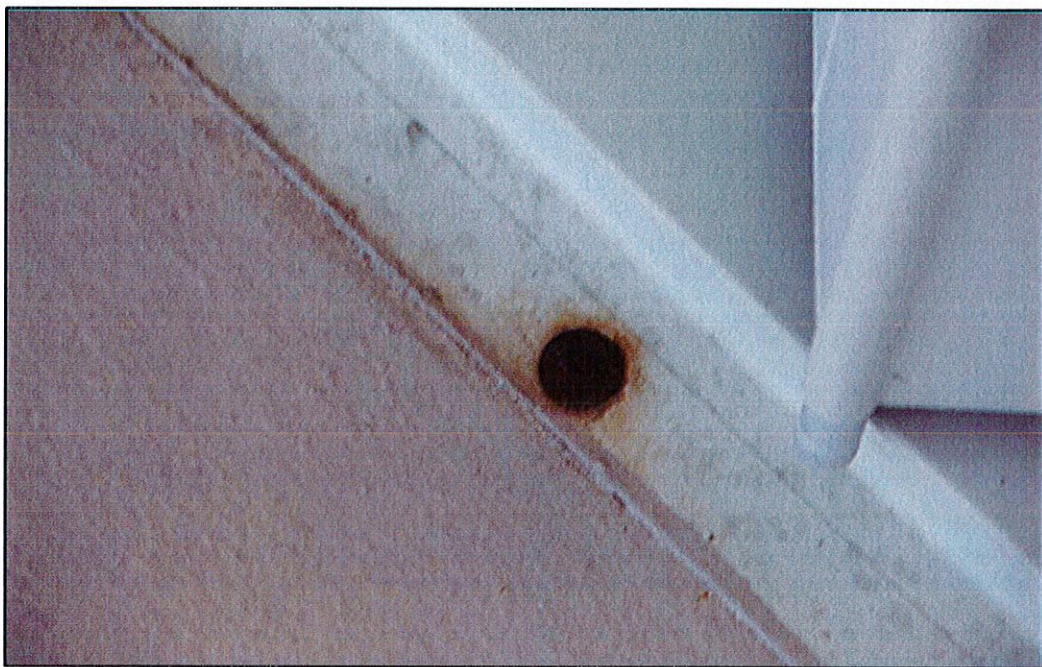
Photo #10. Close up view of deteriorated metal anchors for the hurricane shutters. (Unit 402 shown).
