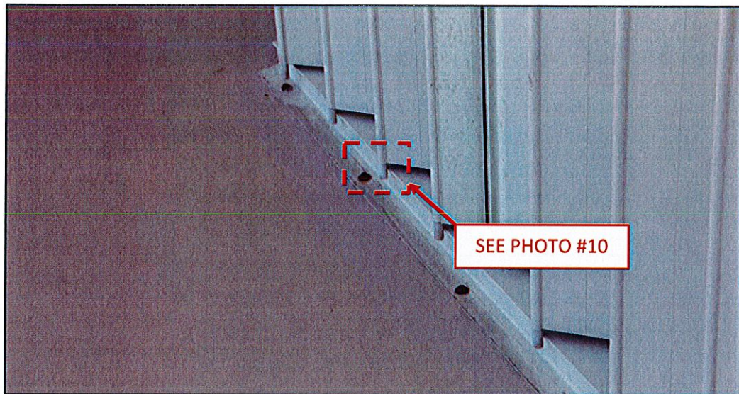
Photo #9. View of deteriorated metal anchors for the hurricane shutters. Observed at several units (Unit 402 shown).
