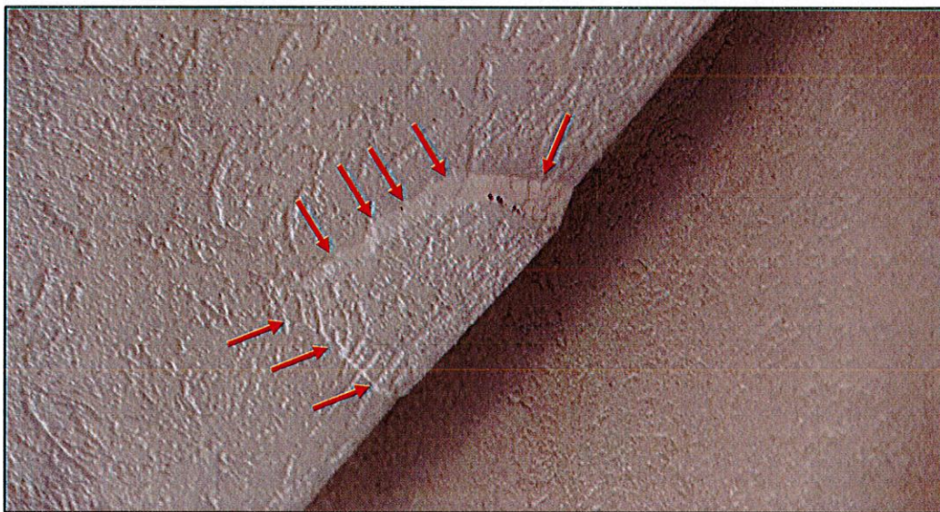
Photo #6. View of exterior stucco finishes with localized bulging (unit 205 front corridor shown).
