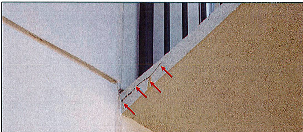
Photo #4. View of imminent spalling of concrete slab edge observed at edge of floor slab (unit 401 front corridor).
