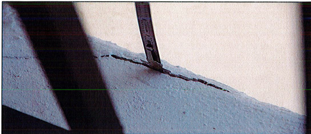
Photo #3. View of imminent spalling of concrete slab edge observed at floor of unit 406 corridor.
