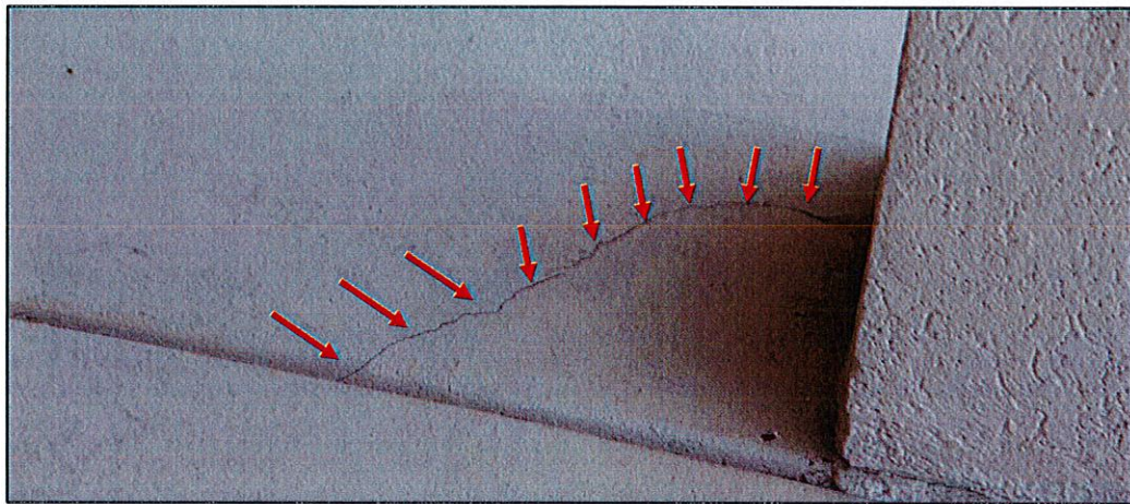
Photo #12. View slab cracks (Unit 203 balcony shown).
