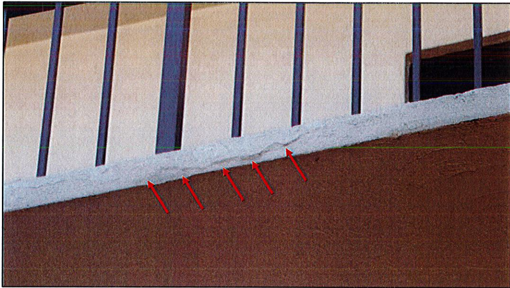
Photo #7. View of deteriorated slab edge finishes, signs of concrete slab spalling due to corroded reinforcing, condition observed at exterior edge of unit 402 corridor.
