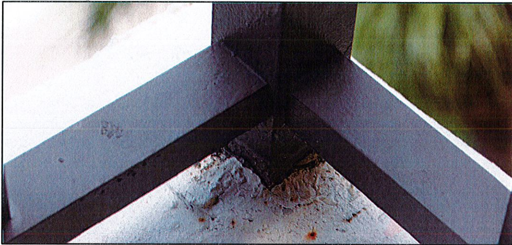
Photo #1. View of post base deteriorated grout and metal post with signs of corrosion damage (unit 501 front corridor).
