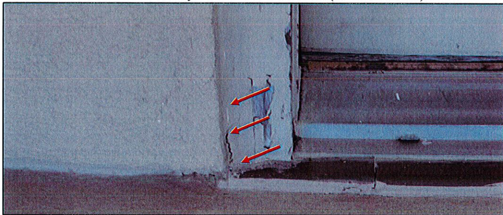
Photo #8. View of deteriorated sealant around the front door of unit 504.
